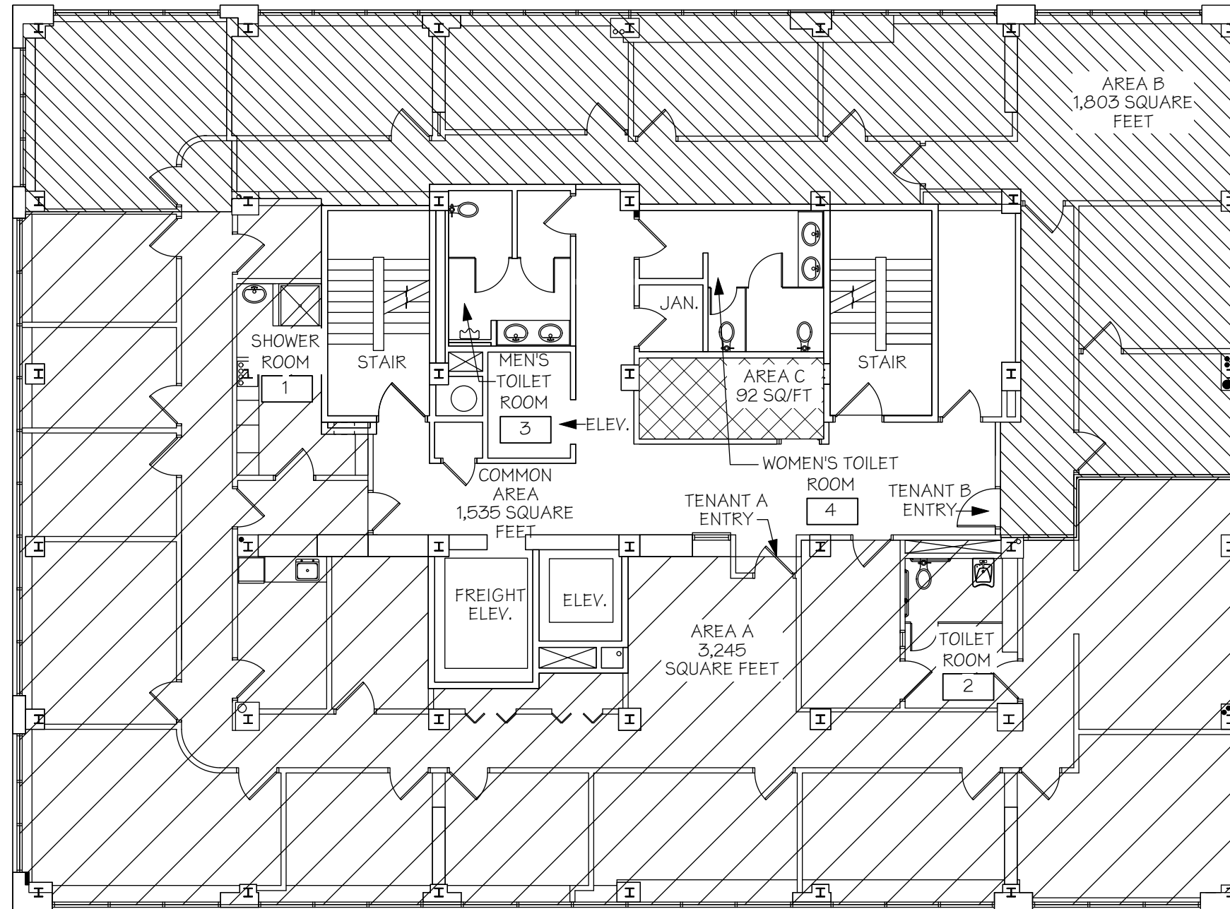
1 THIRD FLOOR PLAN Scale: 3/32" = 1'-0"
